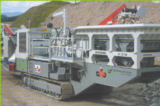
Gipo 130 Combi – independent pre-screen, 1.3m x 1.3m Primary Horizontal Impactor, 6m 2 double deck product screen, suitable for a wide range of applications
